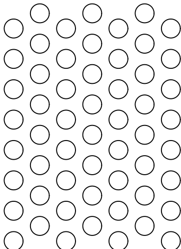
Perforering \varnothing 5 mm. Triangel delning 8 mm. Fri area 35%.
