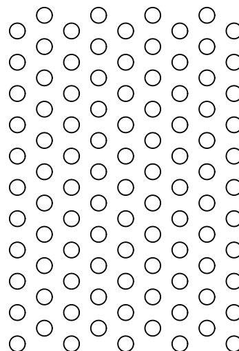
Perforering \varnothing 3 mm. Triangel delning 6 mm. Fri area 23%.
