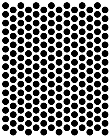
Perforering \varnothing 5 mm. Triangelindelning 6,5 mm. Fri area 53,7%.
