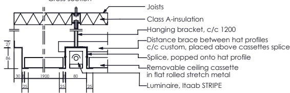
Detail 2 Hat profile Cross-section
