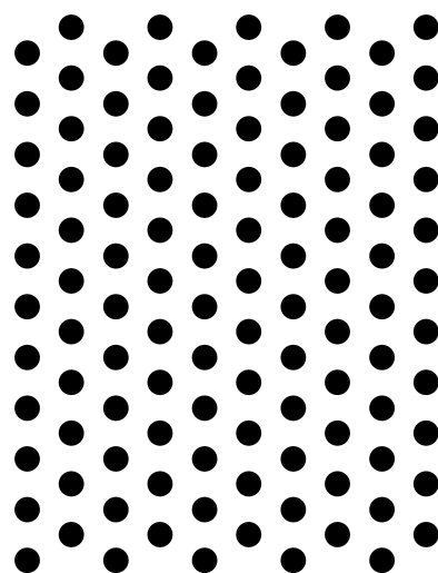
Perforering 3 mm, triangel delning 6 mm. Fri area 23%.
