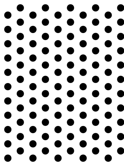
Perforering Ø3 mm. Triangel delning 6 mm. Fri area 23%.
