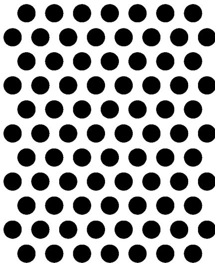
Perforering Ø5 mm. Triangel delning 8 mm. Fri area 35,4%.
