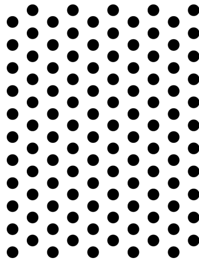
Perforering Ø3 mm. Triangel delning 6 mm. Fri area 23%.
