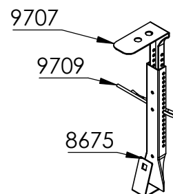
Nonius pendel
